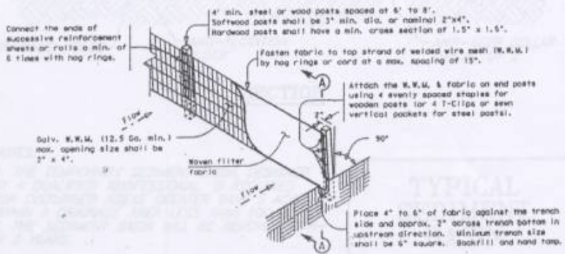
TEMPORARY SEDIMENT CONTROL FENCE
