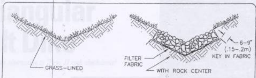
TYPICAL V-SHAPED CHANNEL CROSS-SECTION
