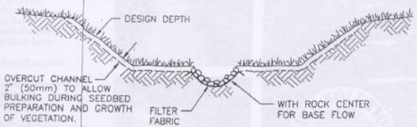
TYPICAL TRAPEZOIDAL CHANNEL CROSS-SECTION
