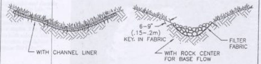
TYPICAL PARABOLIC CHANNEL CROSS-SECTION
